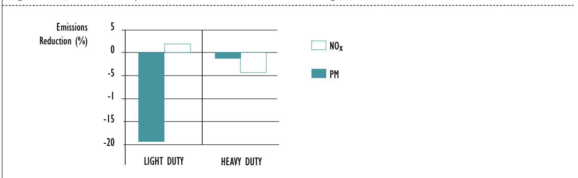
Figure 4: Effect of Density on Exhaust Emissions 855 to 828 kg/m 3
