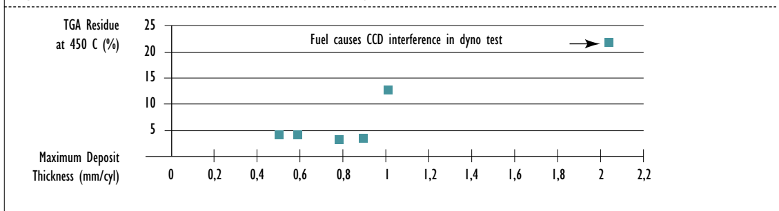
Figure 32: Bis TGA proposed pass/fail limit - 4.0L dynamometer test results
