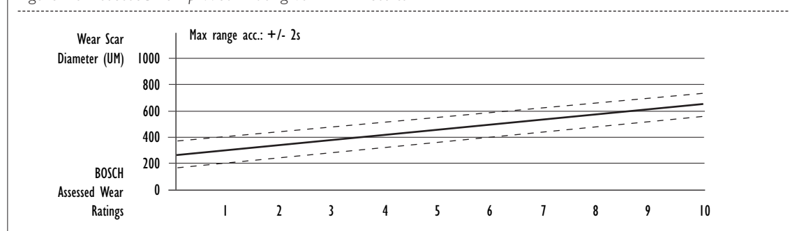
Figure 16: Assessed Pump Wear Rating vs. HFRR Results
