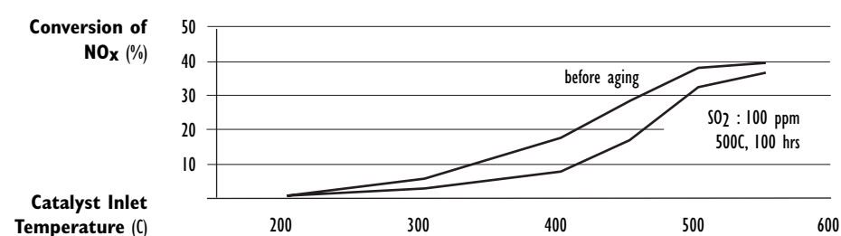
Figure 8: Influence of Sulphur Dioxide Aging on NO x Conversion
