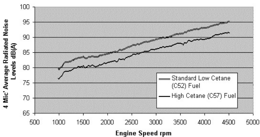
Figure 3: Effect of Cetane on Engine Noise, 52 to 57 CN
