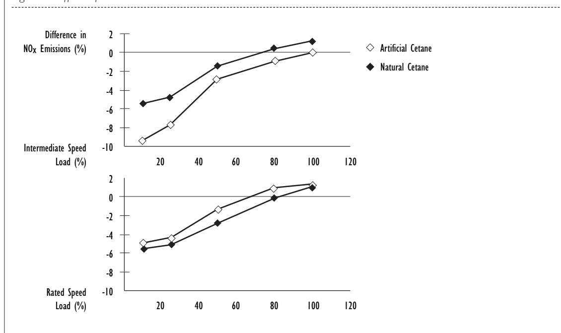
Figure 1: Effect of Cetane on NO x Emissions 50 to 58 CN
