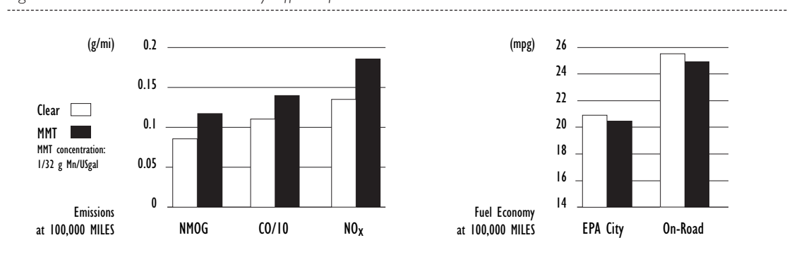
Figure 9: Emission and Fuel Economy Effect of MMT – 1998-99 LEVs
