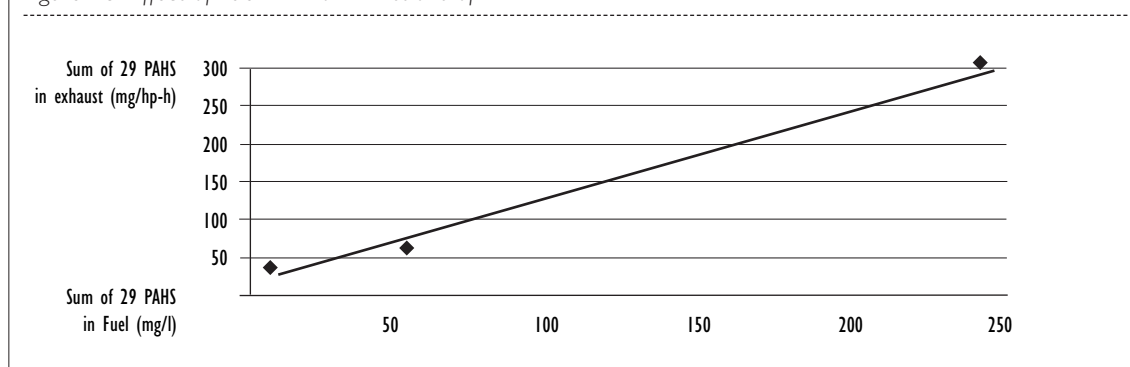
Figure 13: Effect of Fuel PAH on Emissions of PAH
