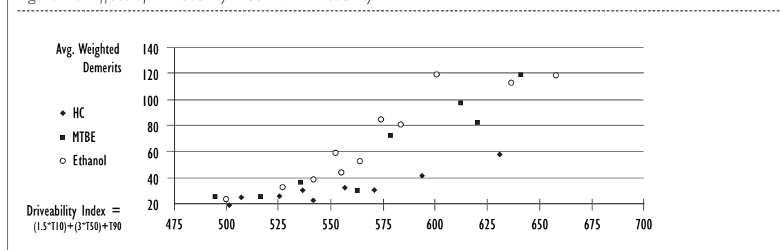
Figure 16: Effect of Driveability Index on Driveability
