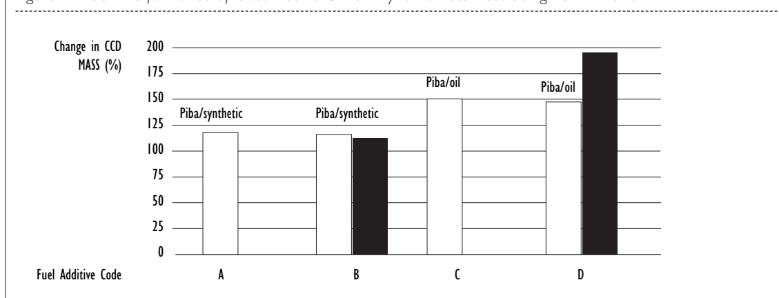
Figure 22: CCD Performance of Gasolines Ford 2.3L Dynamometer Test Using ASTM D6201
