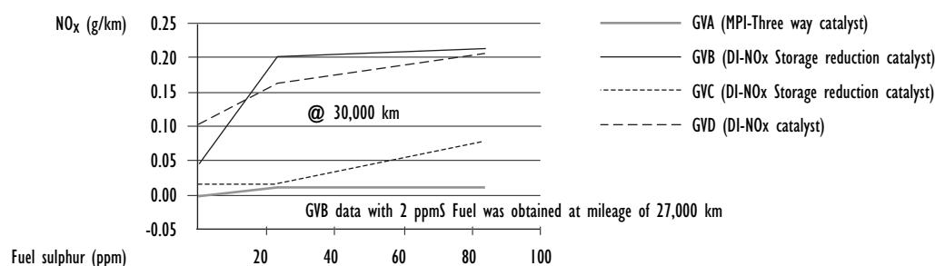
Figure 4: Sulphur effect on Low emission vehicles – Direct Fuel injection engines (Japan Clean Air Program)
