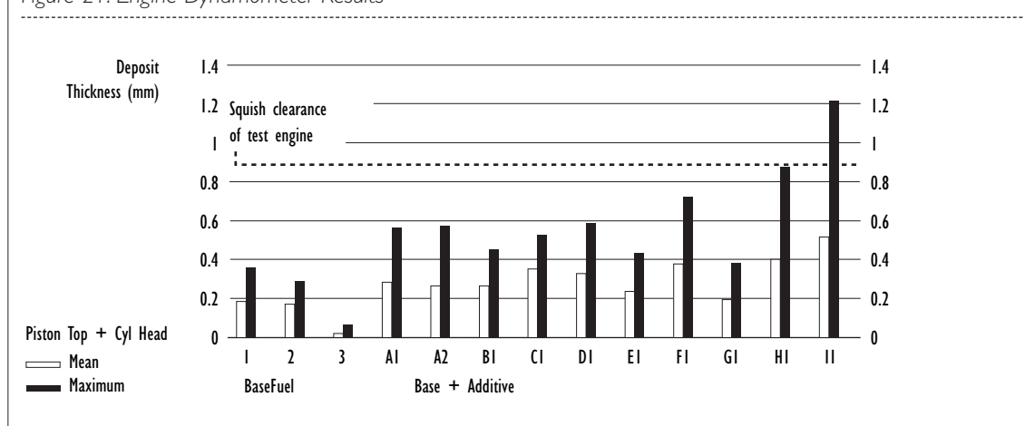
Figure 21: Engine Dynamometer Results
