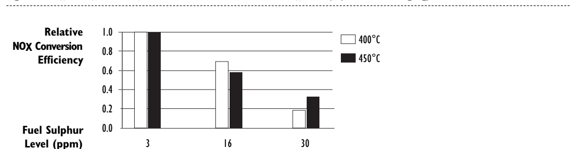
Figure 9: Effect of Fuel Sulfur Level on NO x Conversion Efficiency (150 hours aging)
