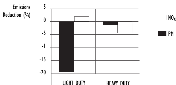
Figure 4: Effect of Density on Exhaust Emissions 855 to 828 kg/m 3
