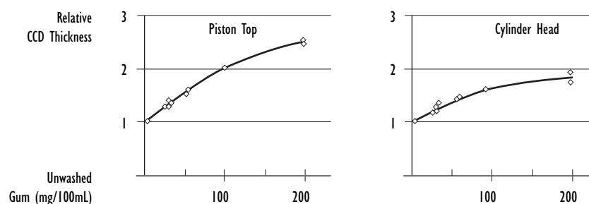
Figure 25: Relationship Between Unwashed Gum and CCD Thickness
