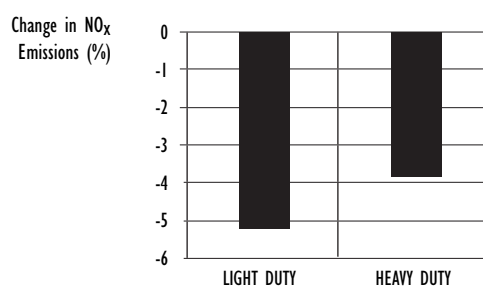
Figure 11: Effect of Total Aromatics on NO x Emissions 30 to 10% aromatics
