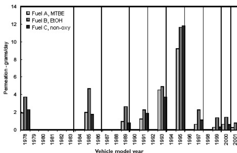
Figure 13: Average Diurnal Permeation of Day 1 & Day 2 (CRC E65 Fleet)
