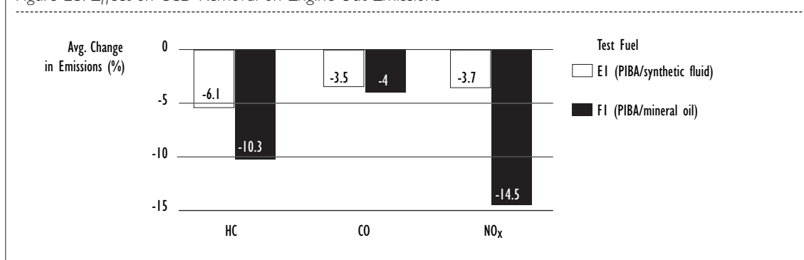
Figure 23: Effect on CCD Removal on Engine-Out Emissions
