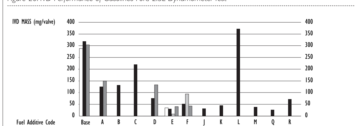
Figure 20: IVD Performance of Gasolines Ford 2.3L Dynamometer Test
