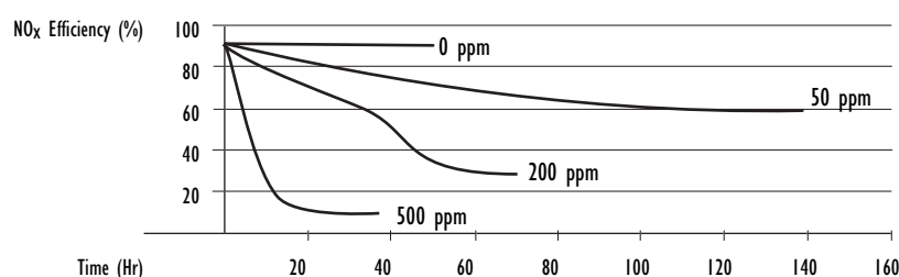
Figure 5: Effect of Fuel Sulphur on Lean NO x Traps Flow Reactor Study
