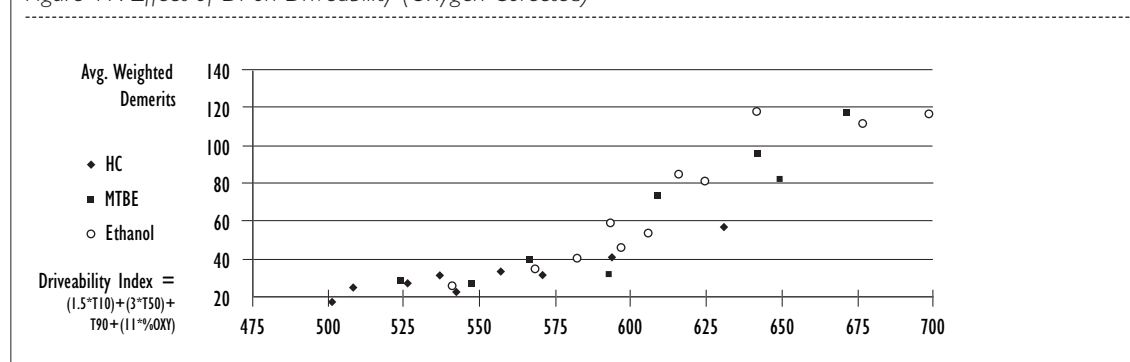
Figure 17: Effect of DI on Driveability (Oxygen Corrected)
