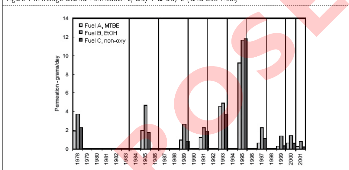
Figure 14: Average Diurnal Permeation of Day 1 & Day 2 (CRC E65 Fleet)
