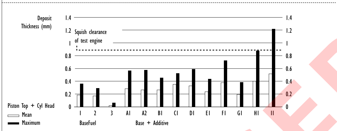
Figure 29: CCD Performance of Gasolines Ford 2.3L Dynamometer Test Using ASTM D6201
